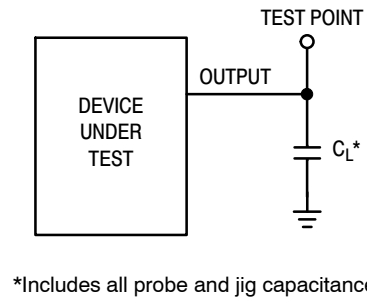
Figure 2. Test Circuit
