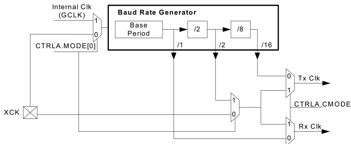
Figure 25-3. Clock Generation
