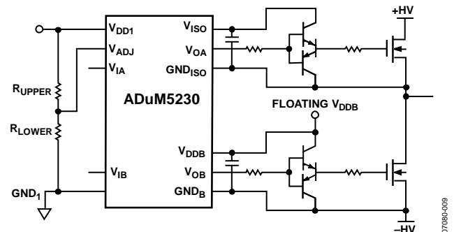
Figure 25. Application Circuit
