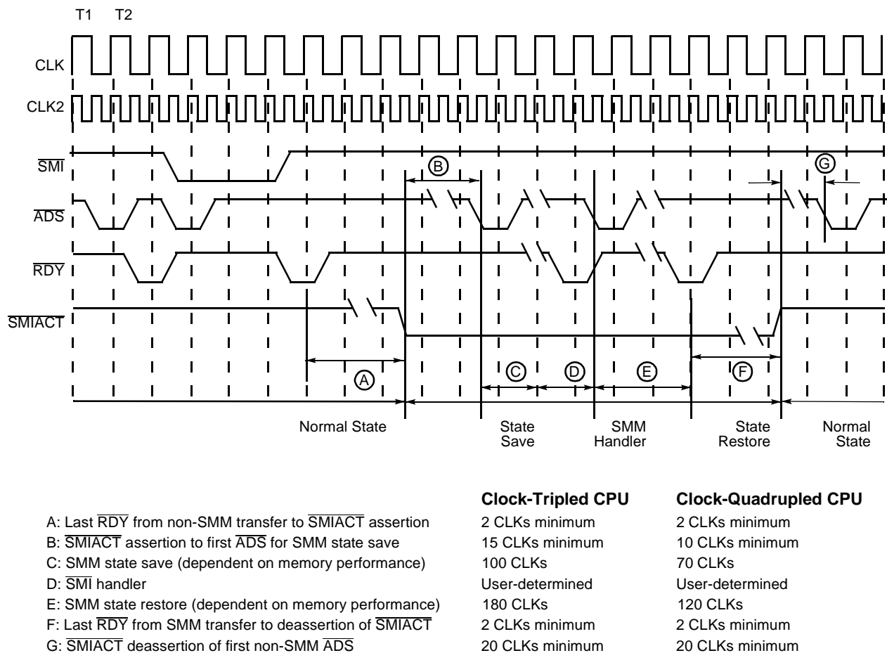
Figure 25. \overline{SMI/ACT} Timing
