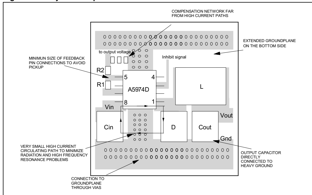
Figure 13. Layout example
