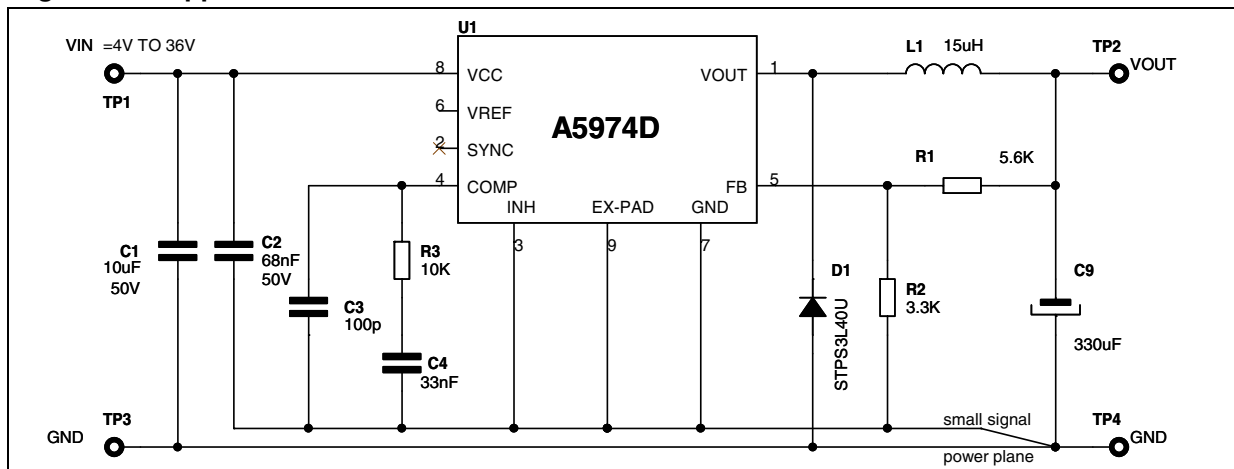
Figure 1. Application schematic
