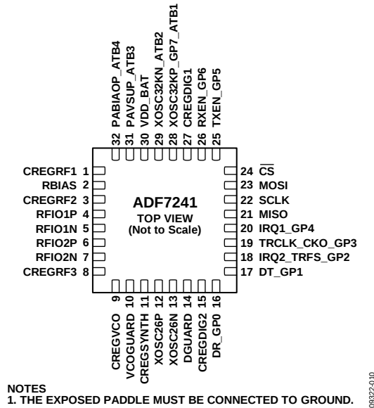
Figure 10. Pin Configuration
