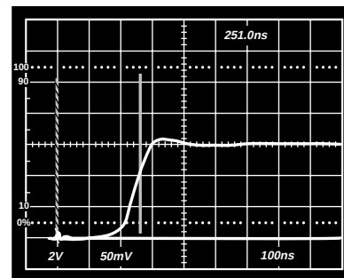
Figure 48. Voltage Output Settling Time
