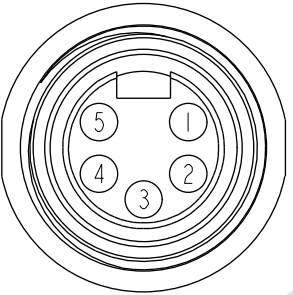
Conn.1 Pin Assignments Front View
