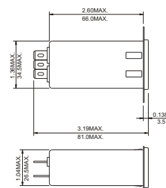
ALL WIRE LEADS 4.0" LONG MIN.
