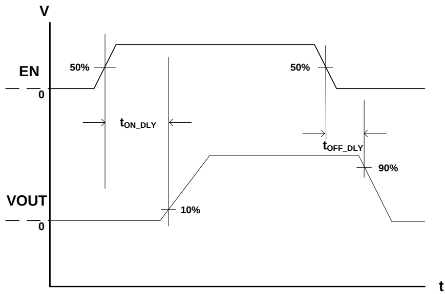
Figure 2. Turn-On/Off Delay
