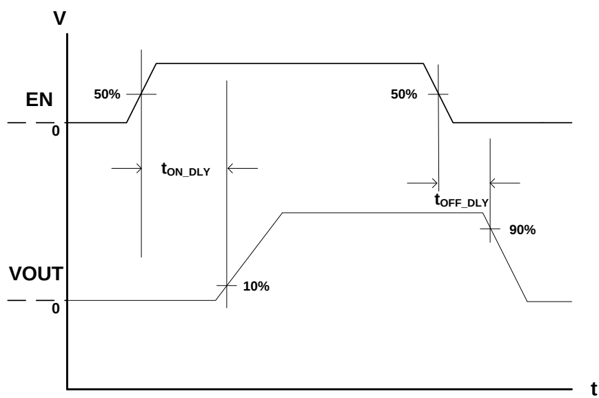
Figure 2. Turn-On/Off Delay
