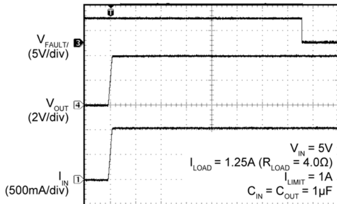
Turn-On Into 25% Overload - 1A I_{LIMIT}
