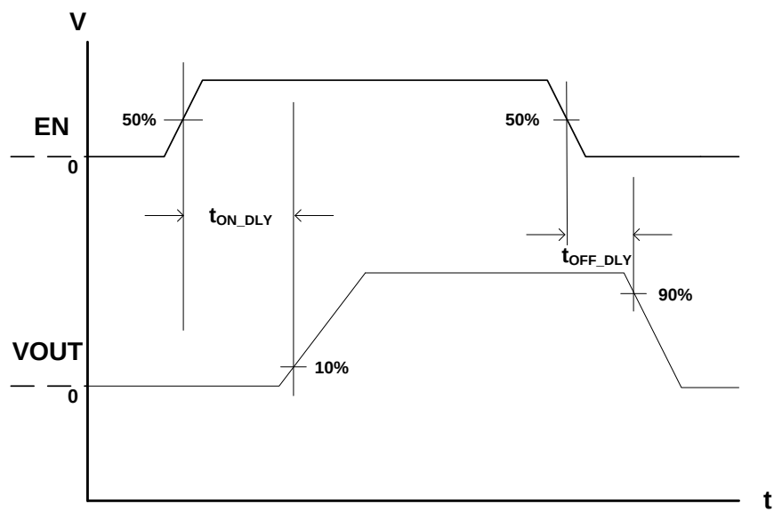
Figure 2. Turn-On/Off Delay
