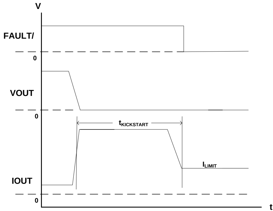
Figure 4. Overcurrent Fault Flag Delay (Kickstart)
