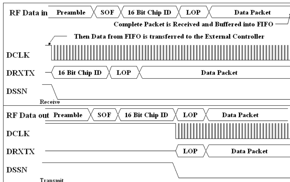
Figure 50: Data Interface Protocol (ID and LOP)
