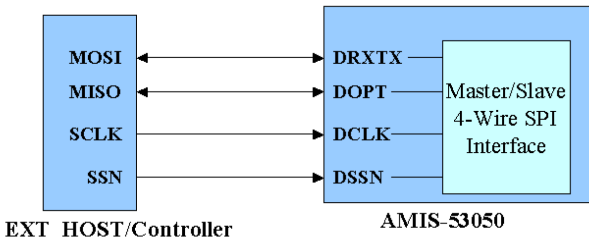
Figure 49: Data Interface Protocol (ID only)
