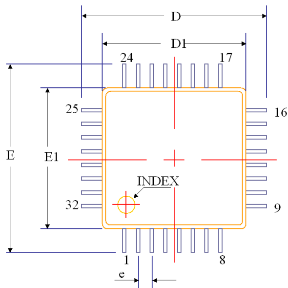
Figure 3: Package
