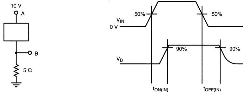
FIGURE 1. Test Circuit 1
