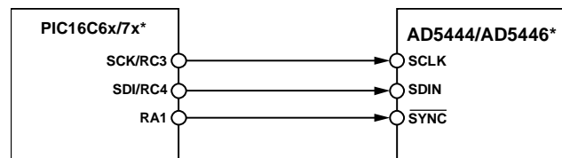
Figure 52. PIC16C6x/7x to AD5444/AD5446 Interface
