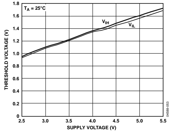
Figure 21. Threshold Voltage vs. Supply Voltage
