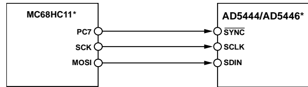
Figure 50. MC68HC11 to AD5444/AD5446 Interface
