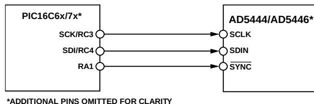
Figure 52. PIC16C6x/7x to AD5444/AD5446 Interface
