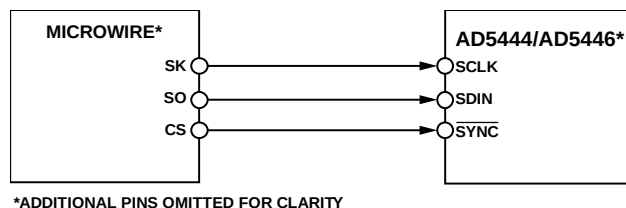
Figure 51. MICROWIRE to AD5444/AD5446 Interface
