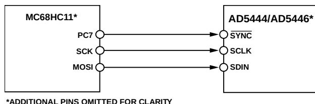
Figure 50. MC68HC11 to AD5444/AD5446 Interface
