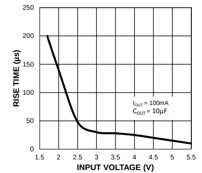
Rise Time vs. Input Voltage (MIC94162/3)
