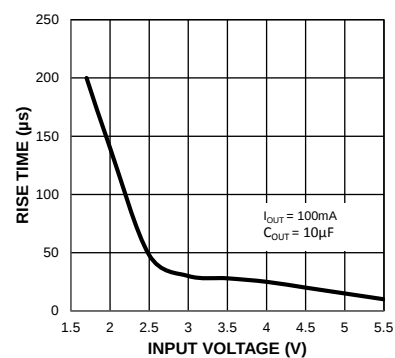
Rise Time vs. Input Voltage (MIC94162/3)
