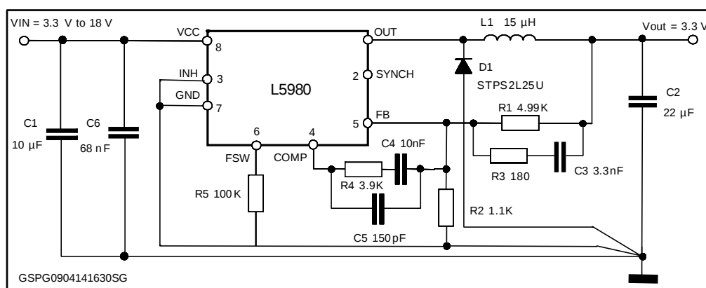
Figure 1: STEVAL-ISA154V1 circuit schematic
