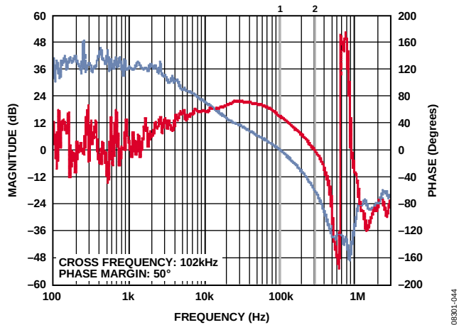
Figure 34. Bode Plot at V_{IN} = 5\text{ V} , V_{OUT} = 1.0\text{ V} , I_O = 3\text{ A} , f_S = 1.2\text{ MHz}
