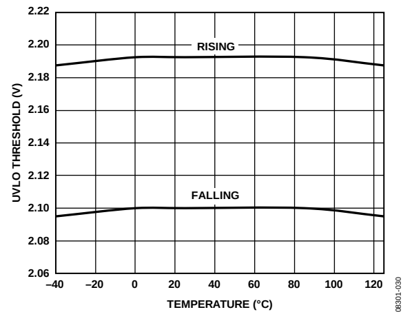
Figure 20. UVLO Threshold vs. Temperature ( V_{IN} = 3.3\text{ V} )
