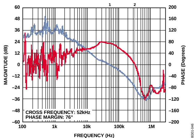
Figure 36. Bode Plot at V_{IN} = 5\text{ V} , V_{OUT} = 2.5\text{ V} , I_O = 3\text{ A} , f_S = 1.2\text{ MHz}
