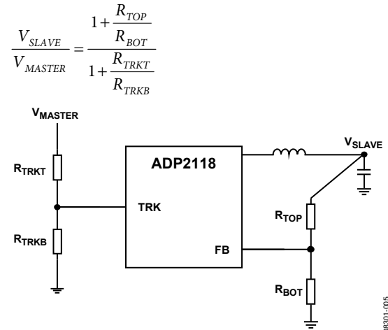
Figure 42. Voltage Tracking
