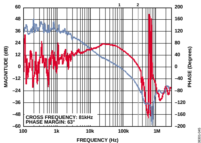
Figure 35. Bode Plot at V_{IN} = 5\text{ V} , V_{OUT} = 1.5\text{ V} , I_O = 3\text{ A} , f_S = 1.2\text{ MHz}
