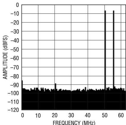
LTC2175-14: 8k Point 2-Tone FFT, f_{IN} = 70\text{MHz} , 75MHz, -1\text{dBFS} , 125Msps
