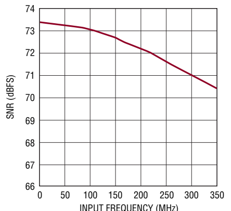
LTC2175-14: SNR vs Input Frequency, -1\text{dB} , 2V Range, 125Msps
