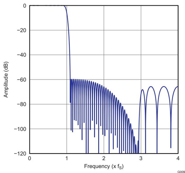
Figure 38. Normal x4 Interpolation Filter Frequency Response
