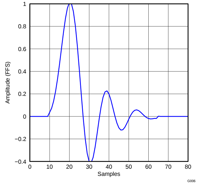
Figure 54. Asymmetric FIR x8 Interpolation Filter Impulse Response, Single Rate
