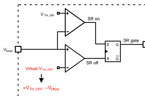
Figure 22. Virtual V_{TH\_OFF}
