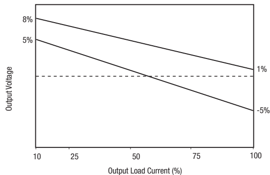
NXJ1S1205MC
