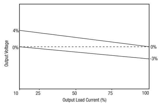
NXJ1S1215MC
