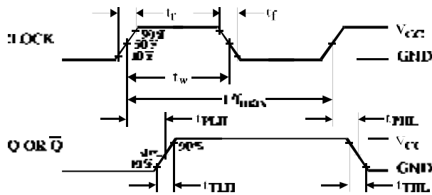
Figure 1. Switching Waveforms
