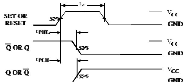
Figure 2. Switching Waveforms
