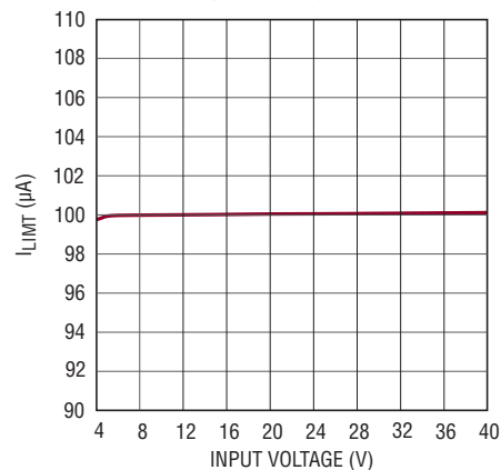
I_{LIMIT} vs Input Voltage
