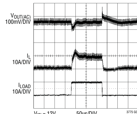
Load Step in Pulse-Skipping Mode
