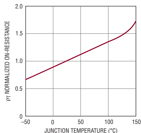
Figure 16. Typical MOSFET R_{DS(ON)} vs Temperature
