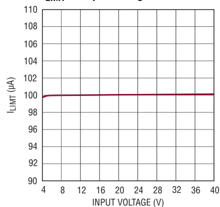
I_{LIMIT} vs Input Voltage
