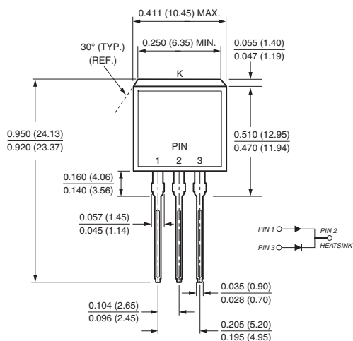
TO-262AA
