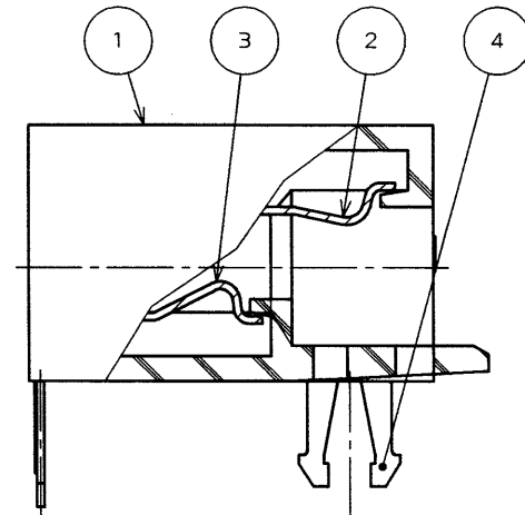
DETAIL (SCALE 5/1)
