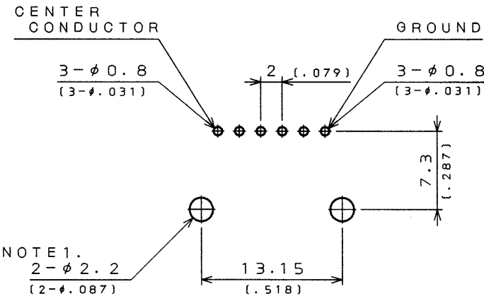
DETAIL (SCALE 5/1)
