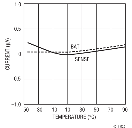
PWM Input Bias Current (OFF)
