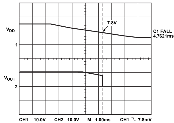
Figure 13. Turn-Off Characteristics
