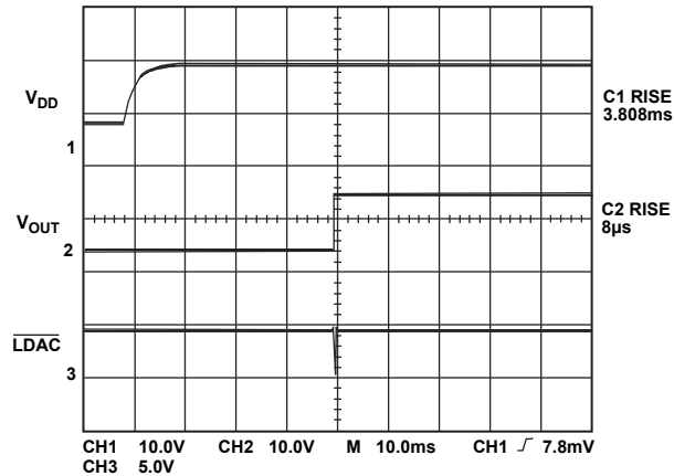
Figure 12. Turn-On Characteristics
