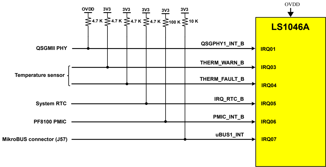
Figure 23. Interrupt assignments
