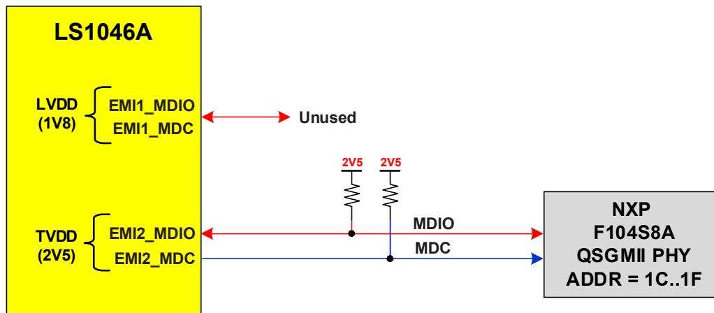
Figure 13. EMI connections
