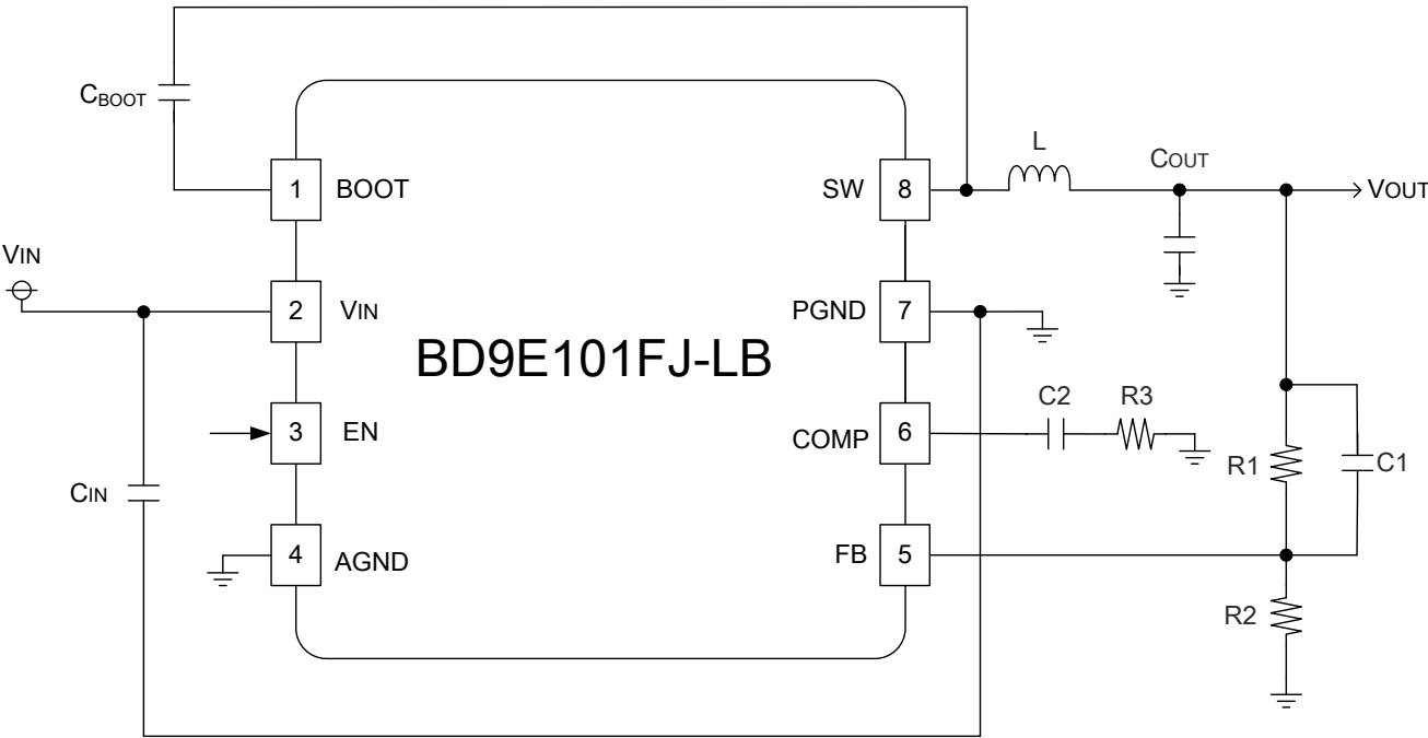
Figure 44. Application Circuit
