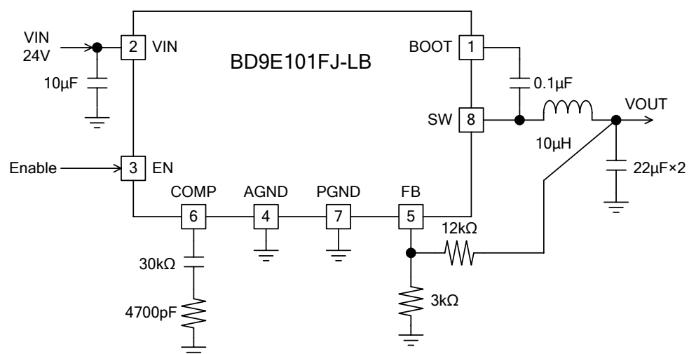
Figure 1. Application circuit
