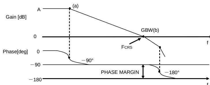
Figure 50. Bode plot
