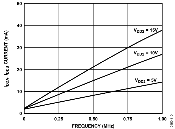
Figure 10. Typical I_{DDVA} , I_{DDB} Supply Current vs. Frequency with 2 nF Load
