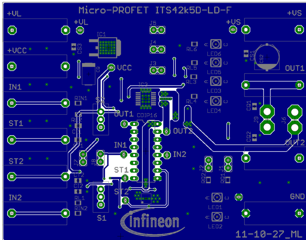
Figure 6 Bottom Layer of ITS42k5D-LD-F Demo board (PG-TSON-10)
