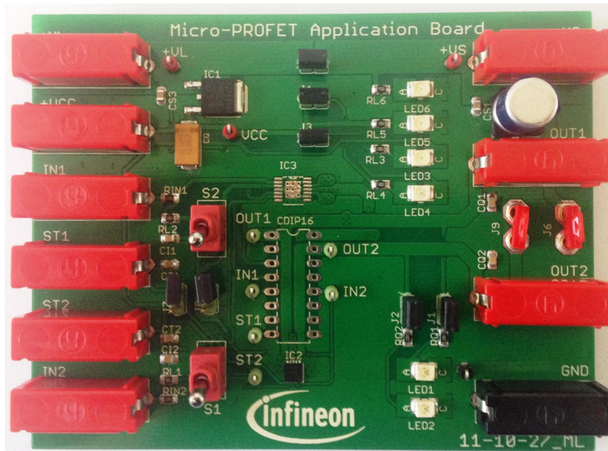
Figure 3 ITS42k5D-LD-F Demo Board (PG-TSON-10)
