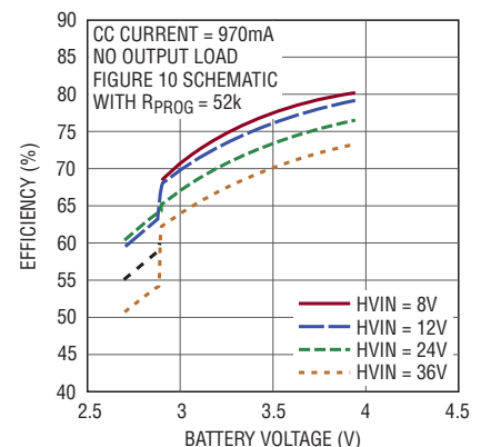
LTC4089 High Voltage Battery Charger Efficiency
