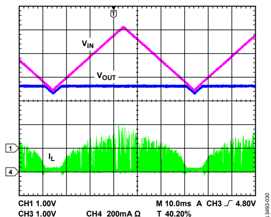
Figure 18. Input Voltage Ramp-Up and Ramp-Down
