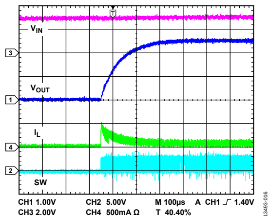
Figure 16. Soft Start, I_{LOAD} = 50\text{ mA}
