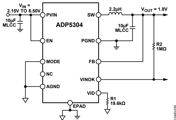
Figure 26. Typical Application Circuit
