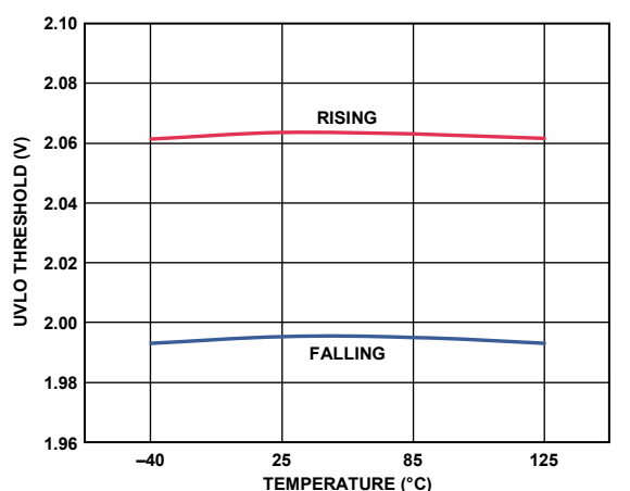
Figure 9. UVLO Threshold, Rising and Falling vs. Temperature
