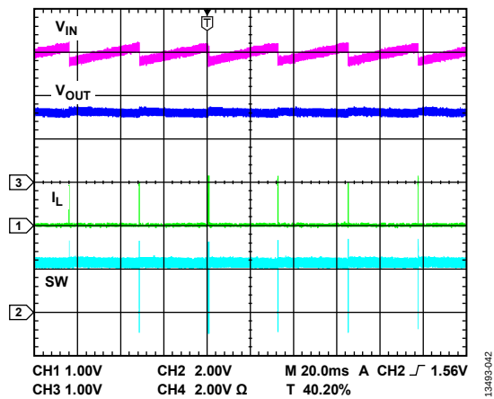
Figure 23. 260 µA Current Source Charge Up, 100 µF Output Capacitor with 100 µA Load Current, and 3.0 V VINOK Threshold
