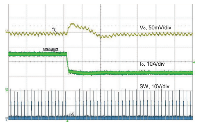
Fig. 49 - Load Release, 12 A to 6 A, 1 A/ \mu\text{s} , t = 10\text{ }\mu\text{s/div}
