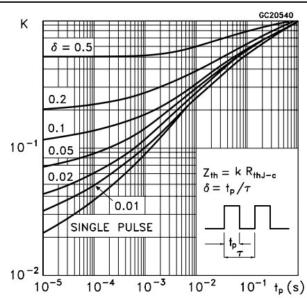
Figure 6. Thermal impedance for TO-220FP
