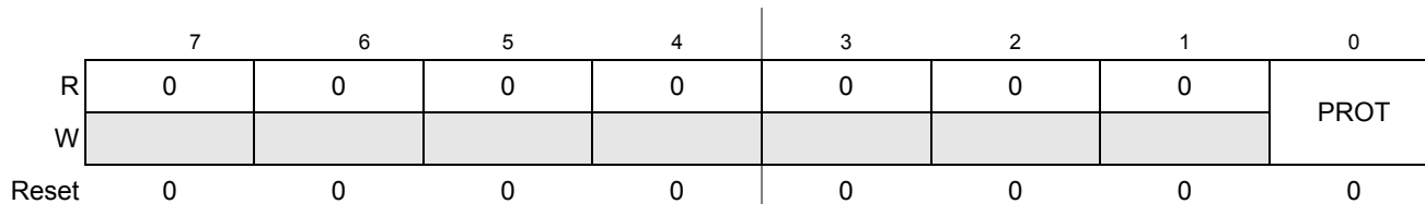
Figure 7-32. S12CPMU_UHV_V6 Protection Register (CPMUPROT)
