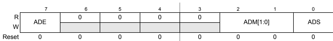
Figure 19-4. SSG attack/decay control register (SSGADC)
