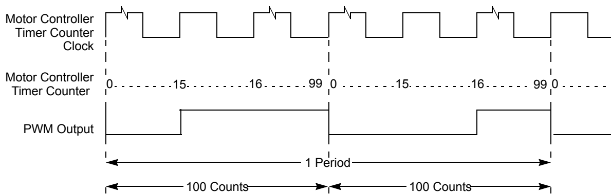
Figure 16-18. PWM Output: DITH = 1, MCAM[1:0] = 01, MCDC = 31, MCPER = 200, RECIRC = 0
