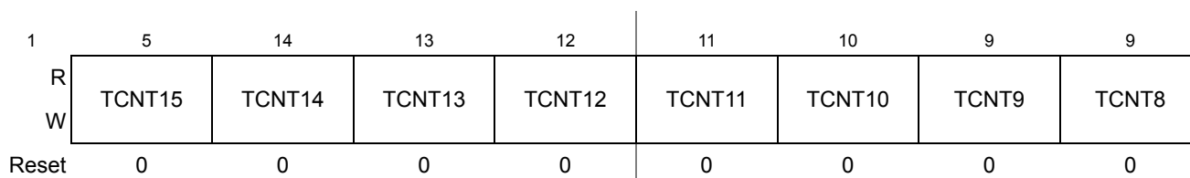
Figure 8-10. Timer Count Register High (TCNTH)
