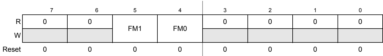
Figure 7-11. S12CPMU_UHV_V6 PLL Control Register (CPMUPLL)
