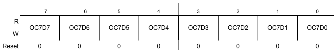
Figure 8-9. Output Compare 7 Data Register (OC7D)
