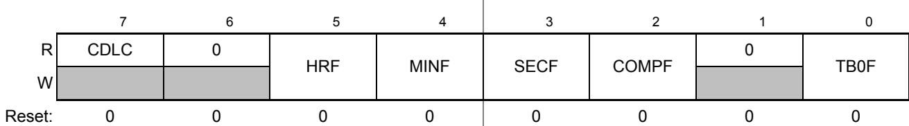
Figure 18-6. RTC Status and Control Register1 (RTCSC1)
