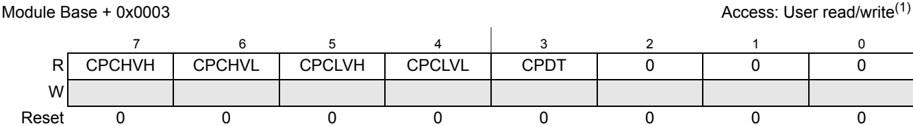
Figure 22-5. CAN Physical Layer Status Register (CPSR)
