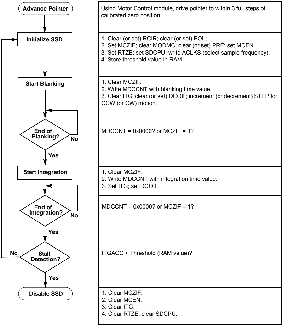
Figure 17-15. Return-to-Zero Flowchart
