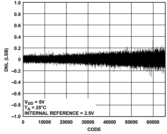
Figure 15. AD5696R DNL
