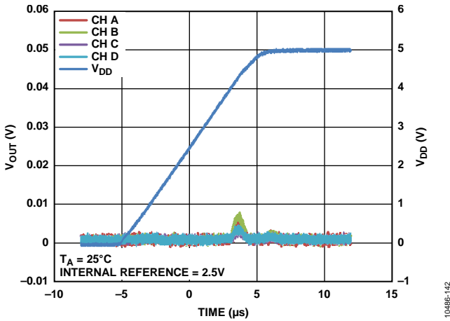
Figure 35. Power-On Reset to 0V
