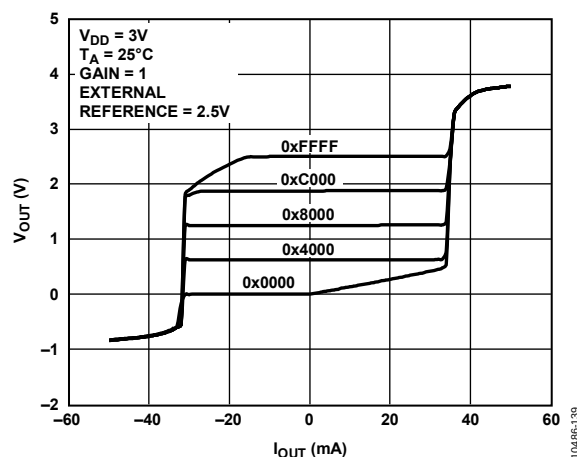
Figure 32. Source and Sink Capability at 3 V
