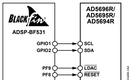
Figure 57. ADSP-BF531 Interface
