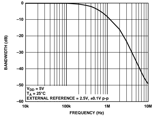
Figure 44. Multiplying Bandwidth, External Reference = 2.5 V, ±0.1 V p-p, 10 kHz to 10 MHz
