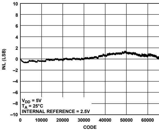
Figure 12. AD5696R INL
