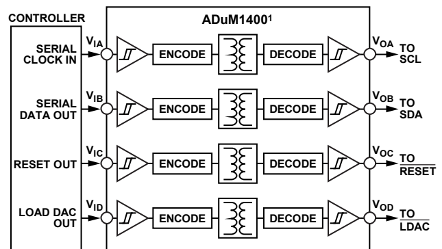
Figure 59. Isolated Interface
