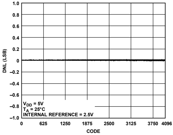
Figure 17. AD5694R DNL
