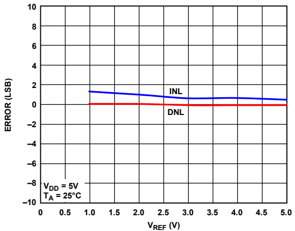
Figure 19. INL Error and DNL Error vs. V_{REF}
